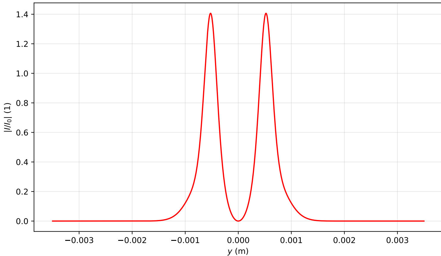
Intensity profile I(x=0, y, z=0.478)/I_0 , \text{Pin}=7.0\text{Pcr} , artificial time
